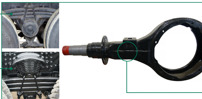
Freightliner/ Sterling Tuftrac or Comparable Suspensions
