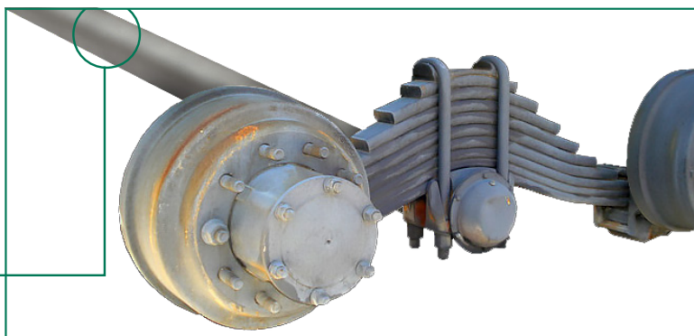
Mack Camel Back or Comparable Suspensions
